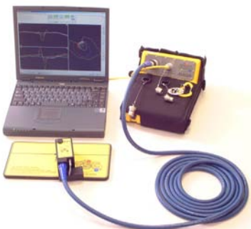
ACFM AMIGO Kit
