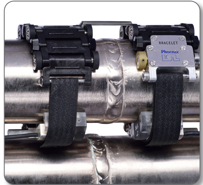
Dual Bracelet configuration scanning double sided phased array on 2" pipe
